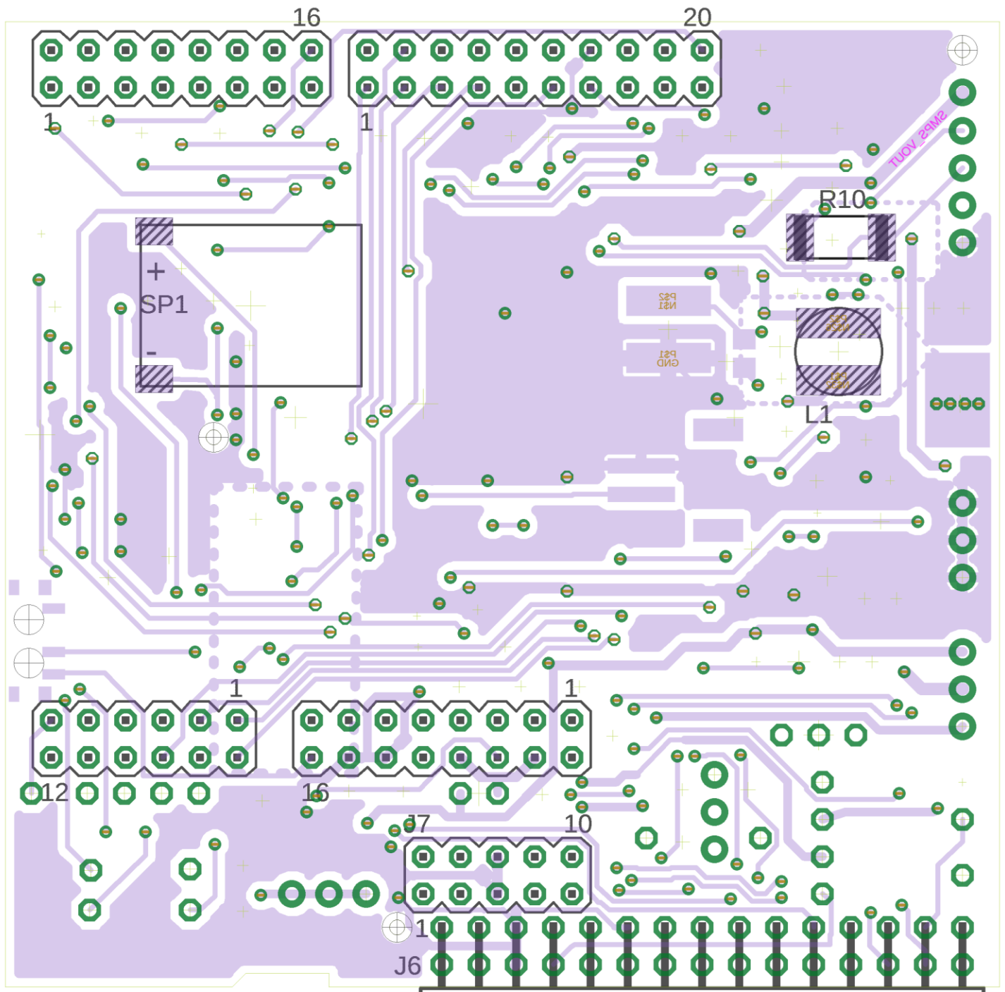
Figure 3. Bottom of PCB
