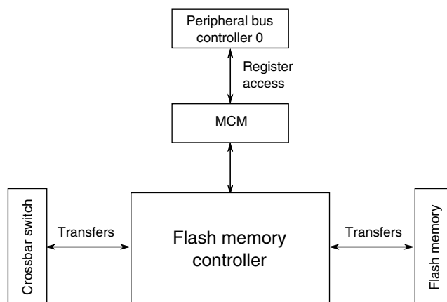
Figure 3-18. Flash memory controller configuration
