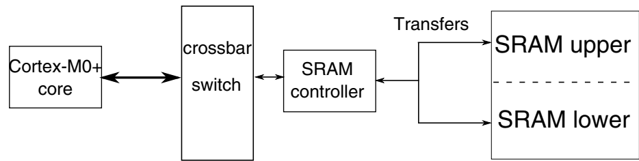
Figure 3-19. SRAM configuration
