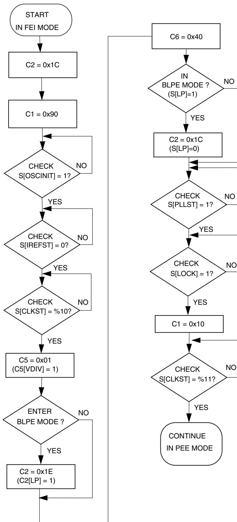
Figure 24-17. Flowchart of FEI to PEE mode transition using an 4 MHz crystal KL25 Sub-Family Reference Manual, Rev. 1, June 2012
